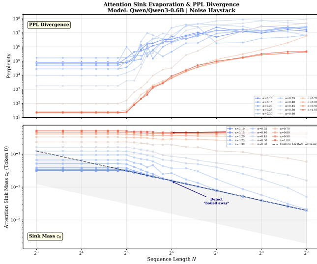
FIG. 11. Attention Sink Probability Mass c_0 vs. Sequence Length N for Selected \alpha . At full capacity ( \alpha = 1.0 ), c_0 \approx 0.44 – 0.51 , far exceeding the uniform baseline 1/N . As \alpha decreases, c_0 undergoes a monotonic, ordered decay, eventually collapsing to the uniform level c_0 \approx 1/N for \alpha \leq 0.30 —the measure-theoretic signature of complete defect evaporation.
