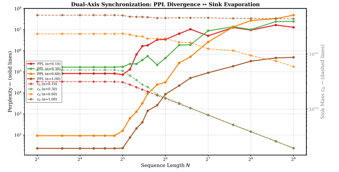
FIG. 12. Dual-Axis Synchronization: PPL Divergence and Sink Evaporation. Solid lines (left axis, log-scale): perplexity vs. sequence length N for \alpha \in \{0.10, 0.30, 0.60, 1.00\} . Dashed lines (right axis, log-scale): corresponding sink mass c_0 . As \alpha decreases, the perplexity explosion and c_0 collapse occur in precise synchrony at the same critical (\alpha, N) locus, directly confirming the causal link between boundary defect evaporation and thermodynamic amnesia.
